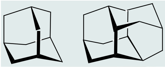
Adamantanoid < 1nm
