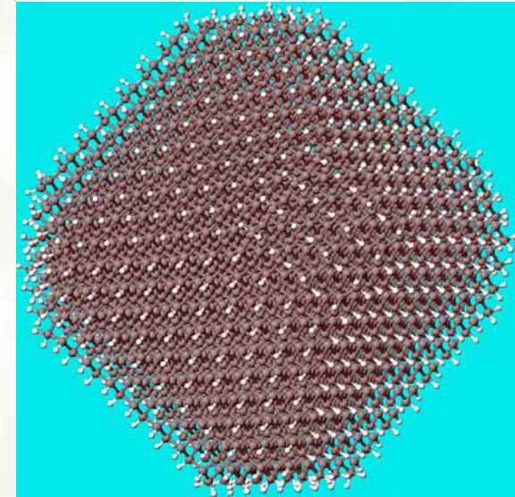
Nanodiamond, 2-100nm
